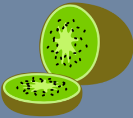
Kiwi
